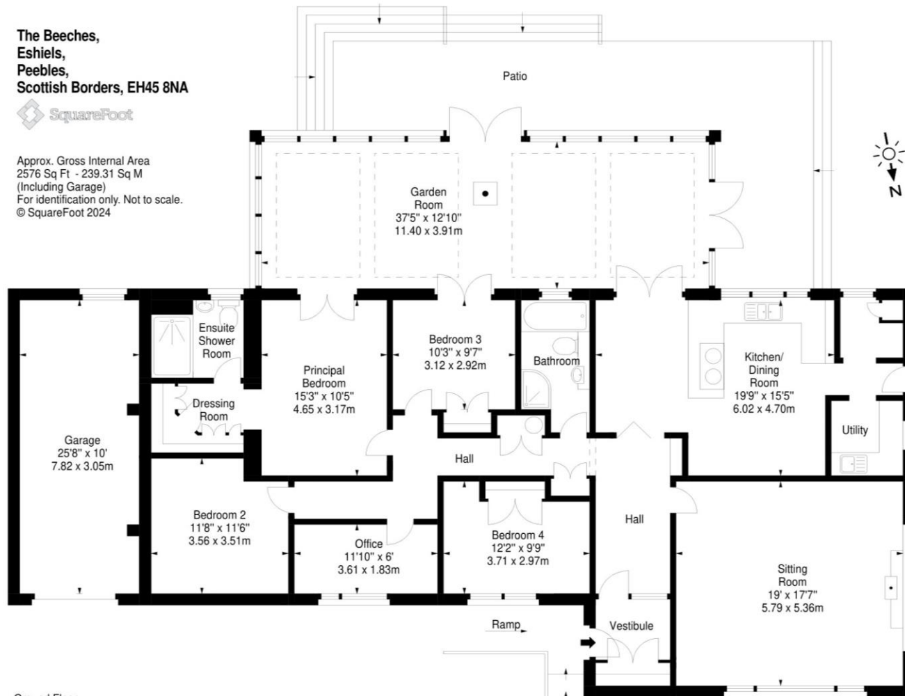
Ground Floor
